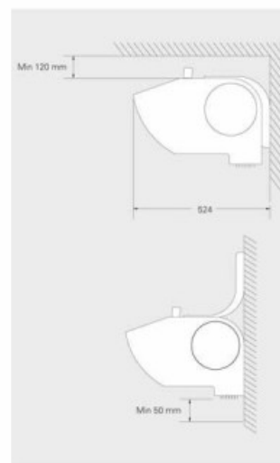
Fig. 1: Distance minimale
