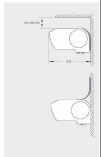
Fig. 1: Distance minimale
